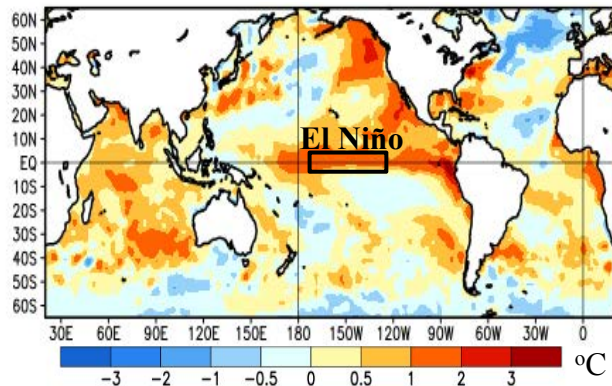
SST Departures ( ^{\circ}\text{C} )
